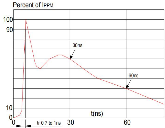
FIG.4: ESD clamping (20kV contact)
