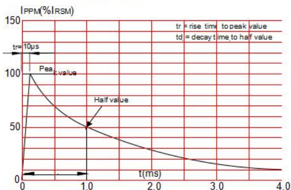
FIG.3: Pulse waveform
