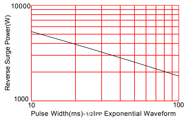
FIG.4: Reverse Power Capability
