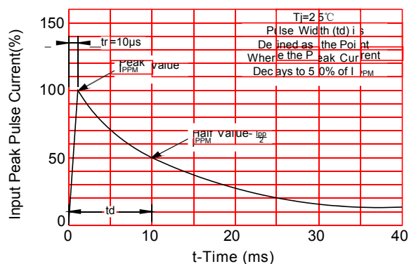
FIG.2: Pulse Waveform
