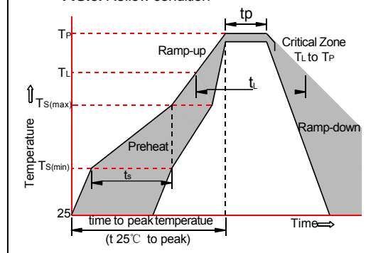
FIG.5: Reflow condition
