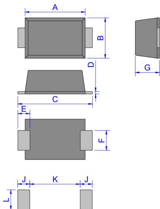
SOD-123FL
