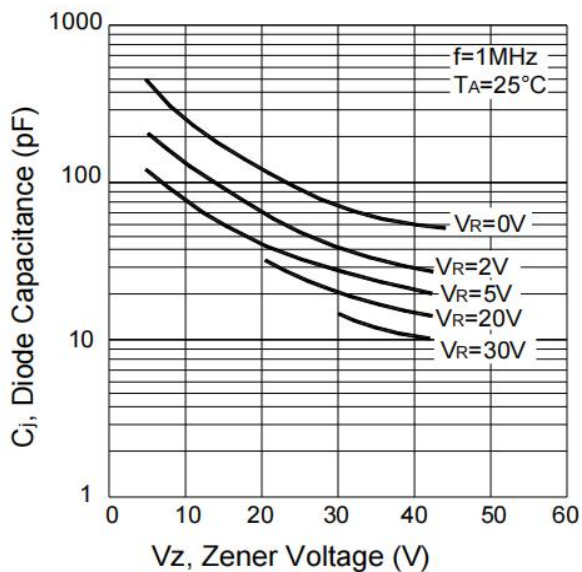
Fig. 3 Junction Capacitance vs Zener Voltage
