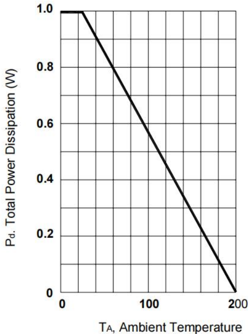
Fig. 1 Power Dissipation vs Ambient Temperature
