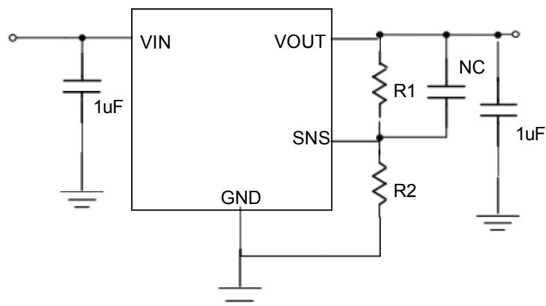
Figure 3: Application circuit of Fixed V OUT LDO with enable and sense functions
