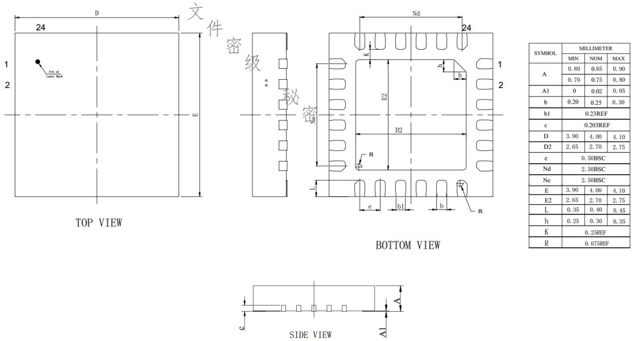
Figure 2-2 HCT6831 封装尺寸
