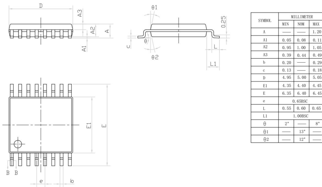
Figure 2-2 HCT6911 封装尺寸
