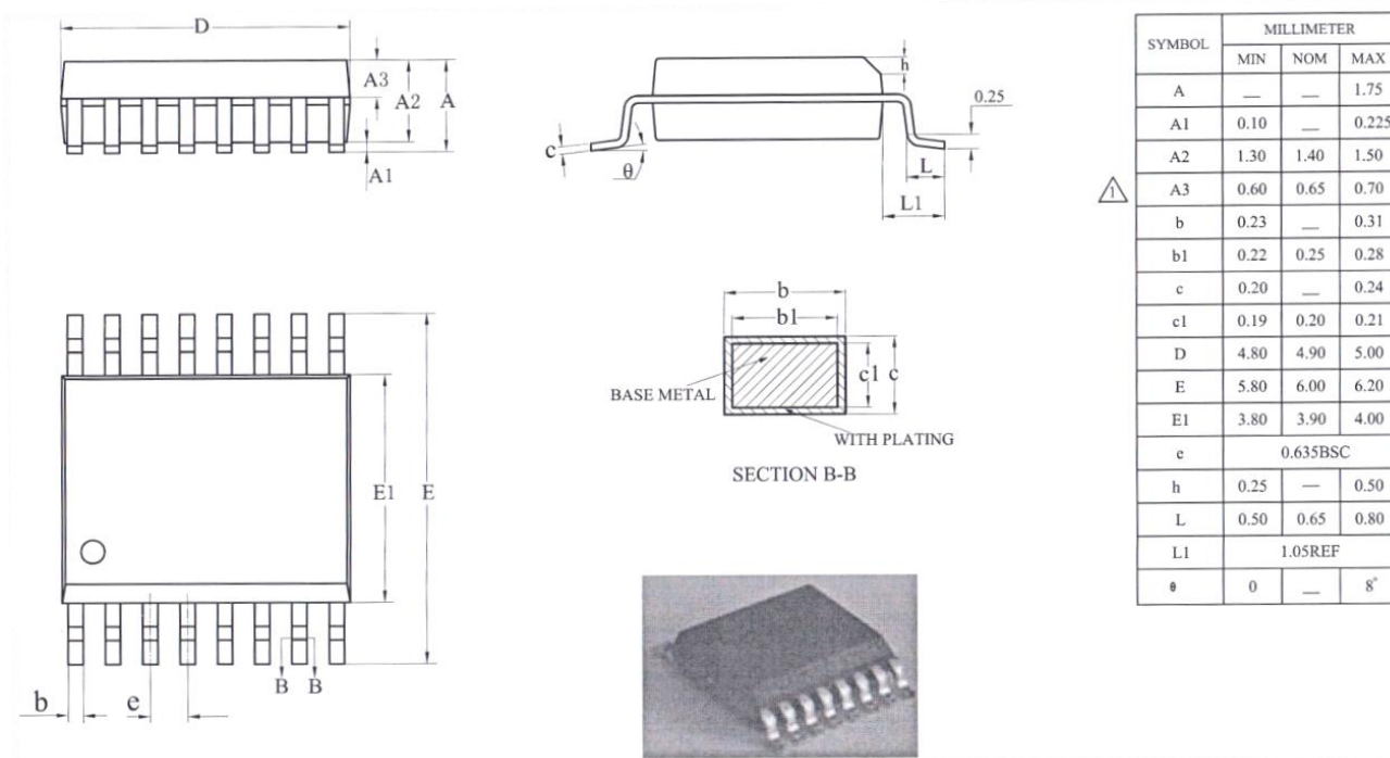
Figure 2-2 HCT6511 封装尺寸
