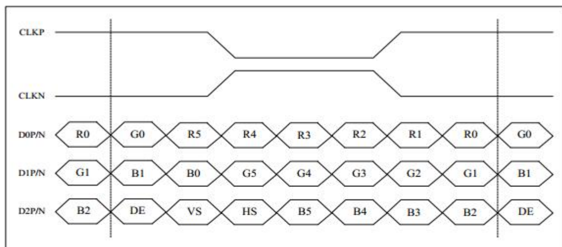
6-bit LVDS input (LVBIT=L, LVFMT=Don)
