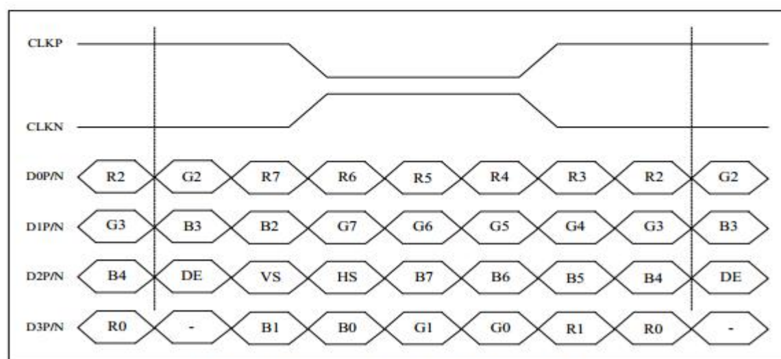
8-bit LVDS input (LVBIT=H, LVFMT=L)
