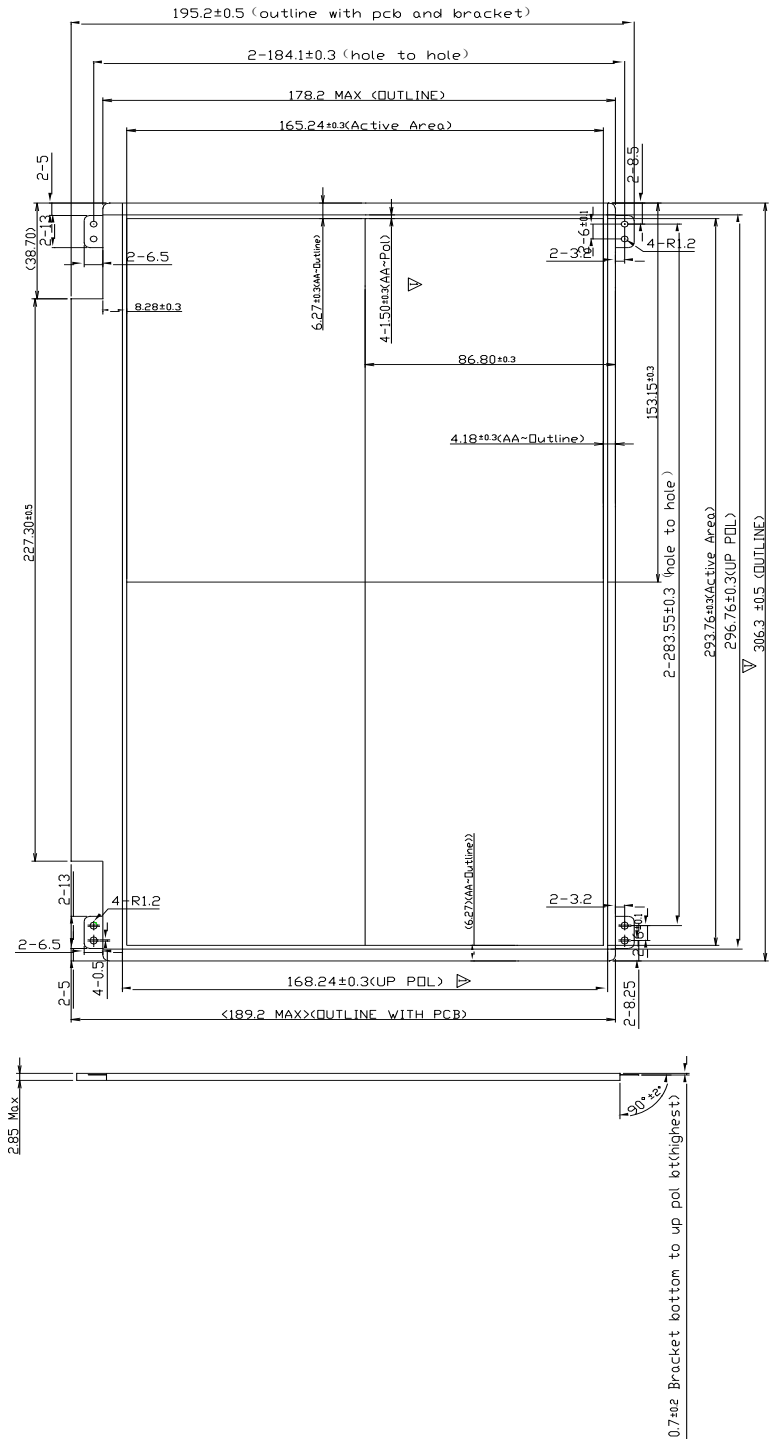
Figure 6. Outline Dimensions (Front view)
