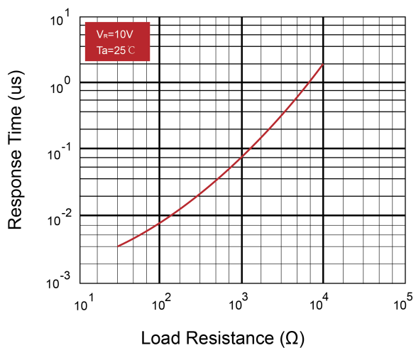
Response Time vs. Load Resistance
