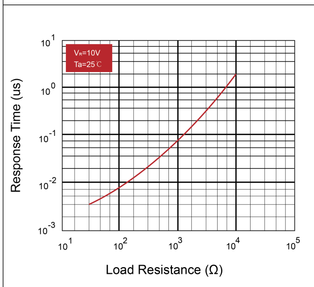
Response Time vs. Load Resistance
