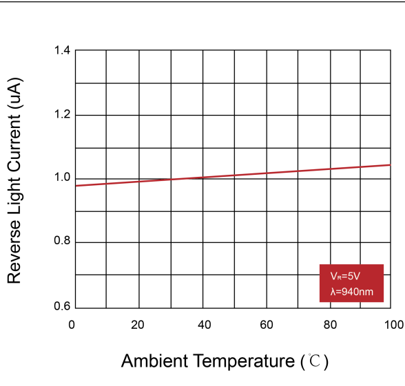
Reverse Light Current vs. Ambient Temperature
