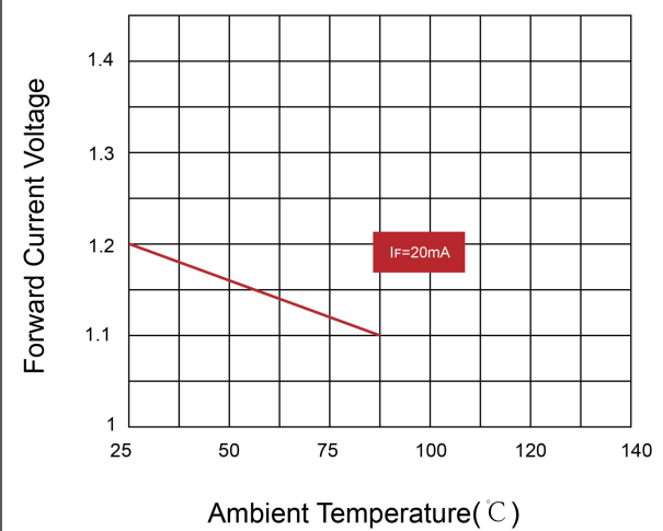
Forward Current vs. Ambient Temperature (°C)
