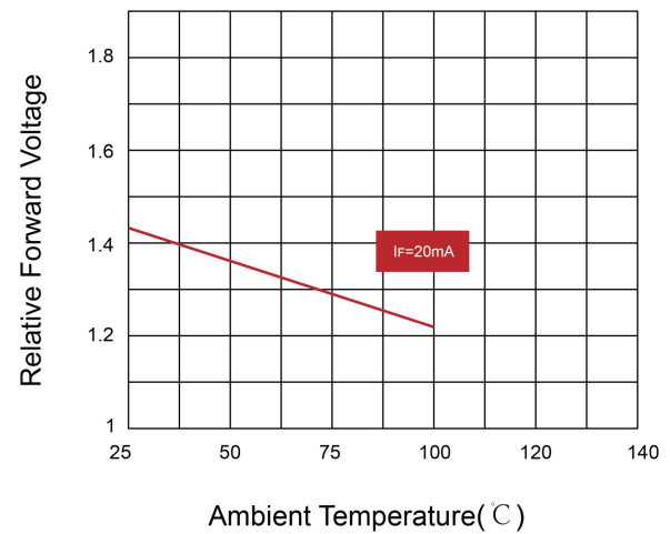
Relative Forward Voltage vs. Ambient Temperature
