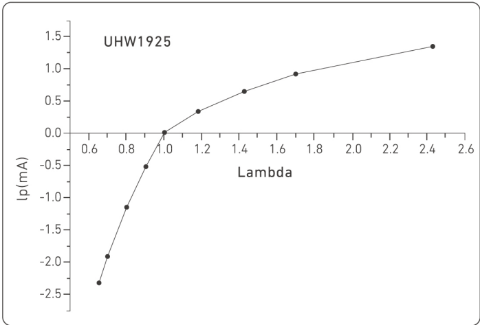
UHW1925 产品典型特征曲线 TYPICAL CHARACTERISTIC CURVE FOR UHW1925
