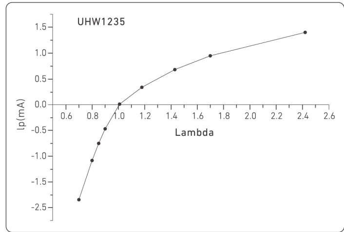
UHW1235 产品典型特征曲线 TYPICAL CHARACTERISTIC CURVE FOR UHW1235
