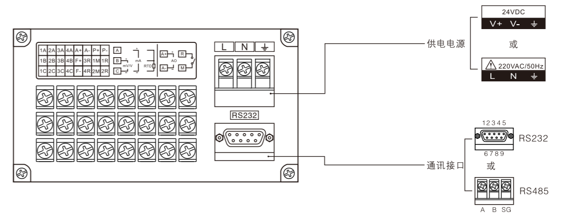
KT100H端子排列
