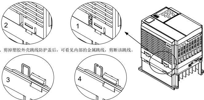
图 7-8 MD310T0.4B、MD310T0.7B、MD310T1.5B、MD310T2.2B、MD310T3.7B、MD310T5.5B 安规电容跳线位置及断开方法
