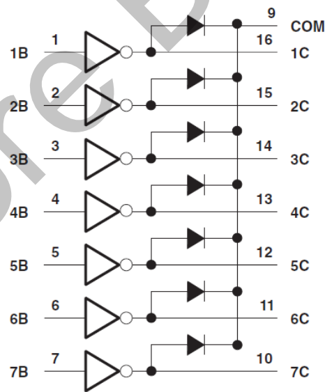
LOGIC DIAGRAM
