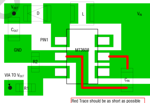
Figure 3. UCB3608 Suggested Layout
