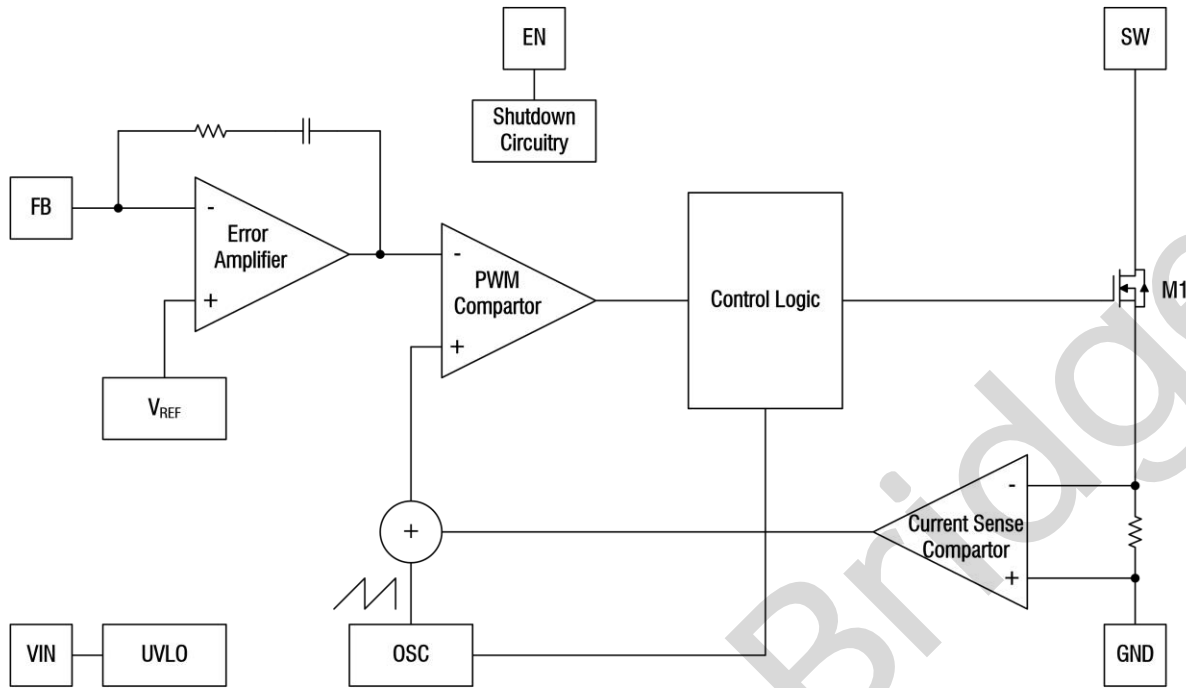
Figure 2. UCB3608 Block Diagram
